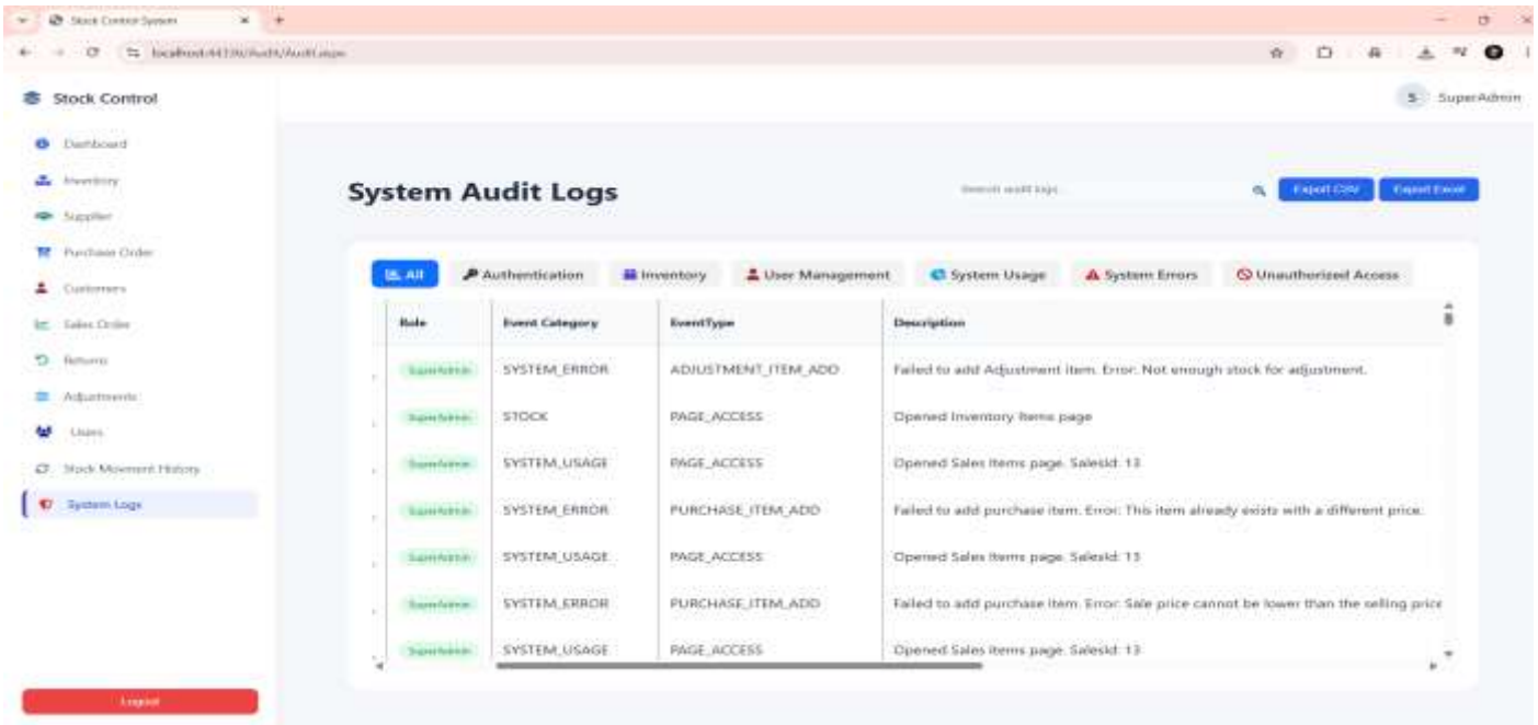
Figure 6.24 – System Audit Logs Page with category filter and export option
