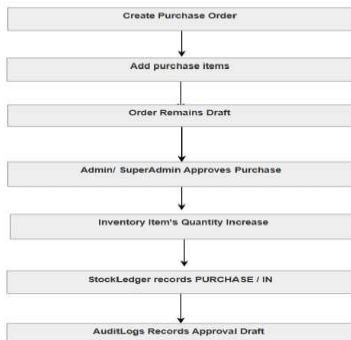
Figure 4.2 – Purchase approval Workflow
